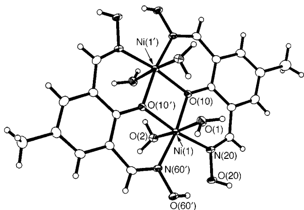
Fig. 3 View of the structure of [\text{Ni}_2(\text{H}_2\text{L}^1)_2(\text{H}_2\text{O})_4]^{2+} with numbering scheme adopted. The perchlorate counter anions and non-coordinating water molecules are omitted for clarity. Primed atoms are related to their unprimed equivalents by the symmetry operation (-x + 1, -y, -z + 1) .
